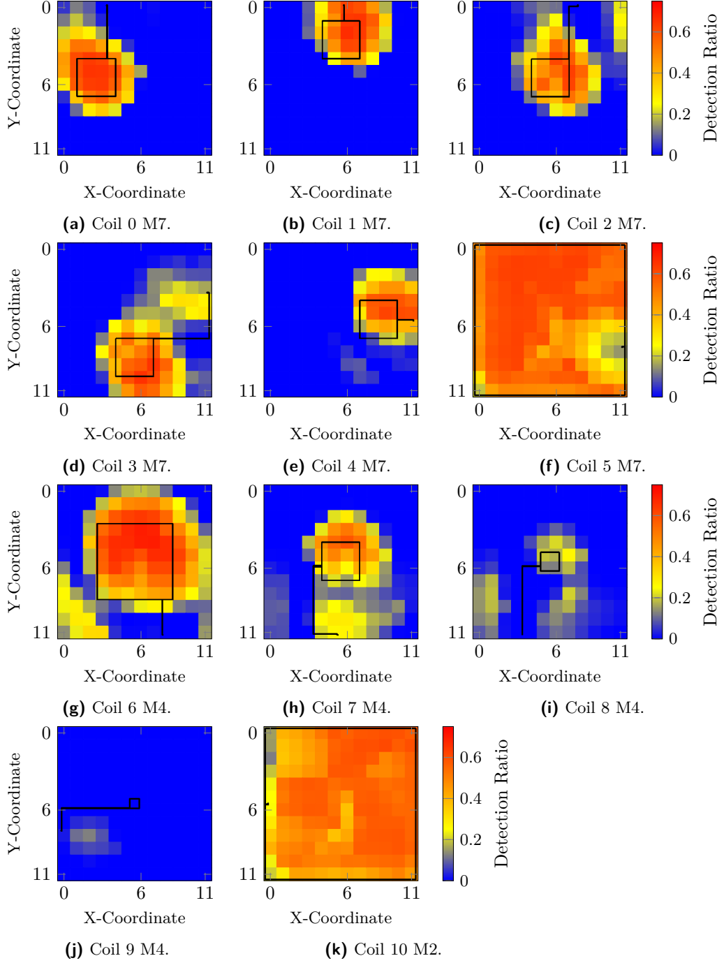
Figure 6: Relative number of experiments E \in \mathcal{E}_{\text{lt}} per location \ell \in L that lead to q_j^{\text{lt}} = 1 , i.e., relative number of fault attempts that were detected by the lt detection register of coil j \in [0, 10] , with coil j depicted in black.
