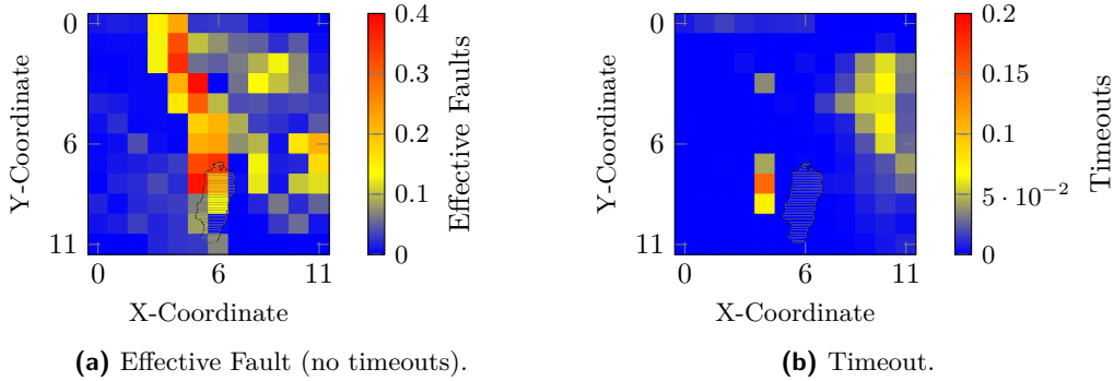
Figure 10: Effective faults with 13 800 experiments per location \ell \in L for target \mathcal{T}_2 with \mathcal{T}_2 shaded and contoured in black.
