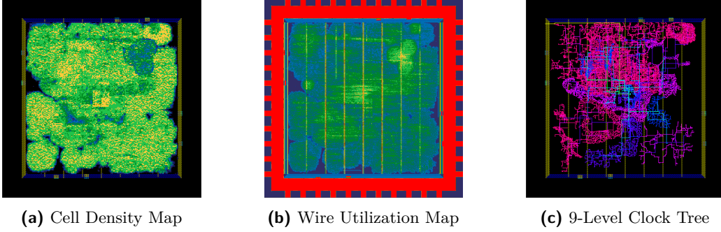
Figure 1: Heatmaps showing cell density, wire utilization and the full clock tree.
