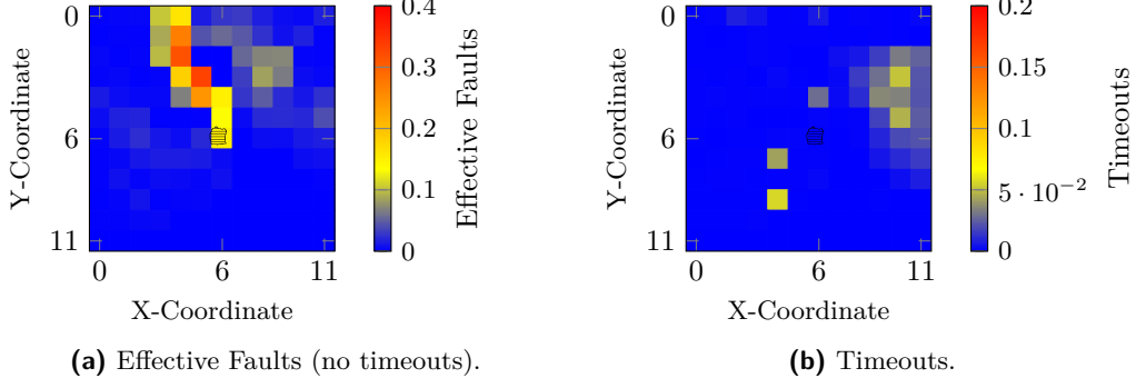
Figure 8: Effective faults with 13 800 experiments per location \ell \in L for target \mathcal{T}_1 with \mathcal{T}_1 shaded and contoured in black.
