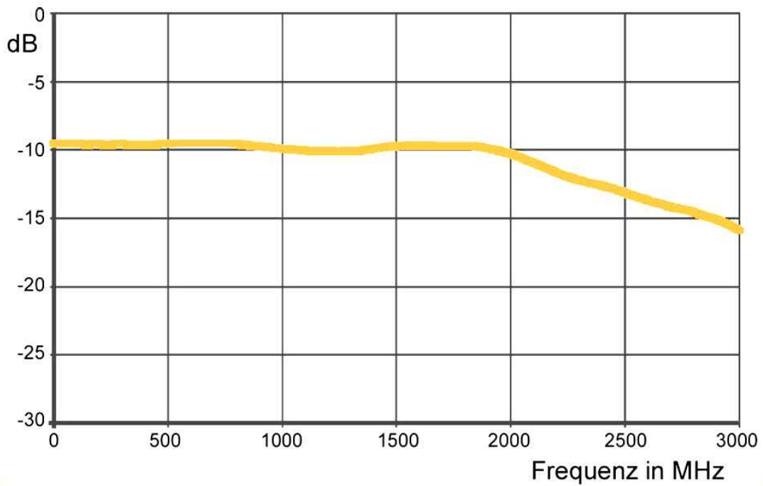
Frequenzgang
