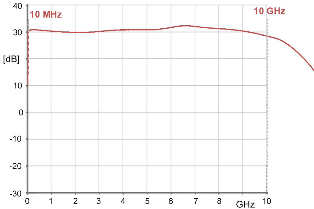
Frequenzgang
