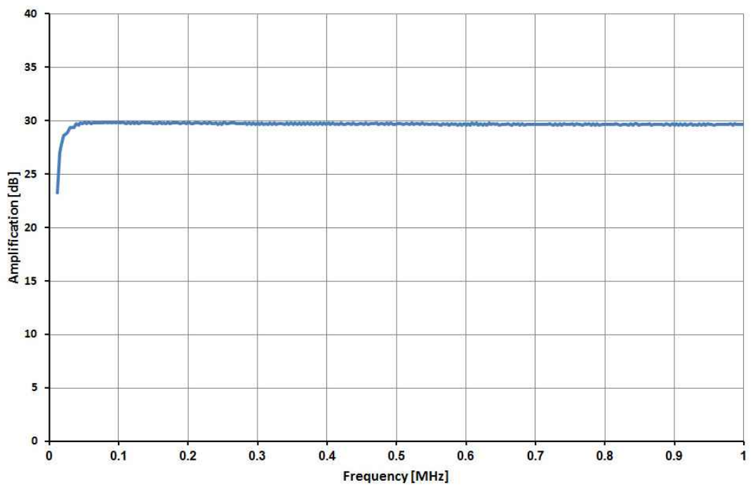
Frequenzgang (Detail)
