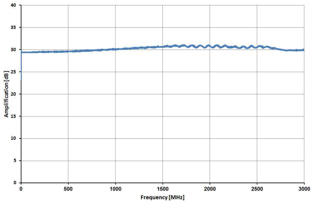
Frequenzgang
