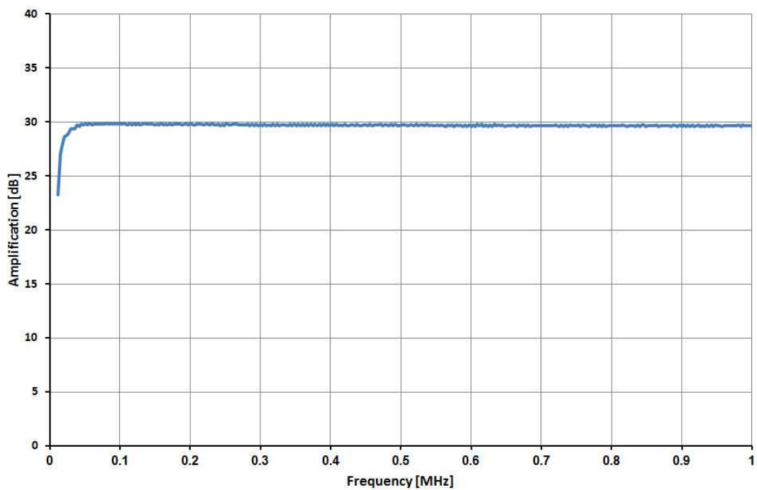
Frequenzgang (Detail)
